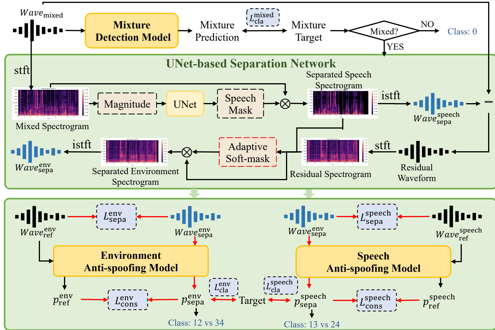
b) Separation-Enhanced Joint Learning Framework
