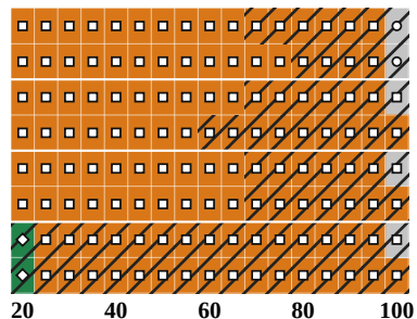
Code
