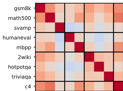
Raw Fisher cosine
