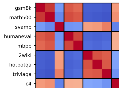
Residual log-Fisher cosine
