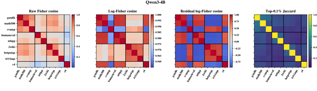
Figure 3: Capability regions in gradient space for Qwen3-4B: pairwise similarity of per-benchmark gradient signatures under four metrics (raw Fisher cosine, log-Fisher cosine, shared-component-removed log-Fisher cosine, top-0.1% coordinate Jaccard). Black lines separate the math, code, QA, and control blocks.
