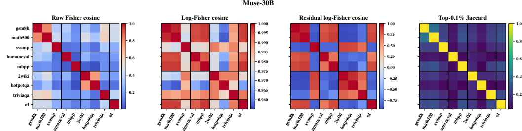
Figure 14: Capability regions in gradient space for Muse-30B: pairwise similarity of per-benchmark gradient signatures under four metrics (raw Fisher cosine, log-Fisher cosine, shared-component-removed log-Fisher cosine, top-0.1% coordinate Jaccard). Black lines separate the math, code, QA, and control blocks.
