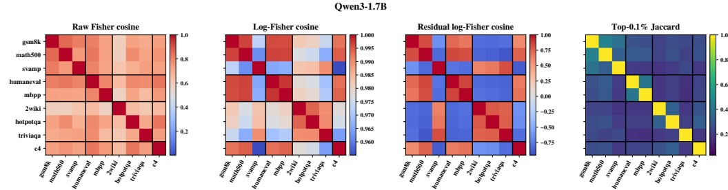
Figure 7: Capability regions in gradient space for Qwen3-1.7B: pairwise similarity of per-benchmark gradient signatures under four metrics (raw Fisher cosine, log-Fisher cosine, shared-component-removed log-Fisher cosine, top-0.1% coordinate Jaccard). Black lines separate the math, code, QA, and control blocks.
