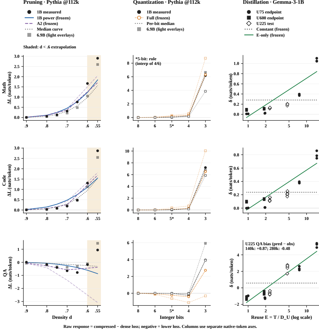
Figure 2: Capability-conditioned compression responses and frozen predictions, one source per arm. Left: pruning of Pythia-1B at step 112k (measured, filled circles) with the frozen shared power form (Eq. 3), the per-density regression A2, and the source-free median development curve; the 6.9B source at the same stage is overlaid in grey and the extrapolated density 0.55 is shaded. Middle: per-channel quantization of the same sources at the integer bit-widths with the frozen per-bit regression (hollow) and the per-bit median (dotted); the 5-bit point is the fixed interpolation rule and guide lines are visual only. Right: distillation of Gemma-3-1B, signed transfer \delta_c against the reuse count E ; endpoint pools U75 and U600 (fit) and the unseen pool U225 (test) with the frozen constant and reuse-count forms and the QA bias at the two budgets. Points are measurements; lines are development fits frozen before the test points were measured. Native nats per token; separate axes per column.
