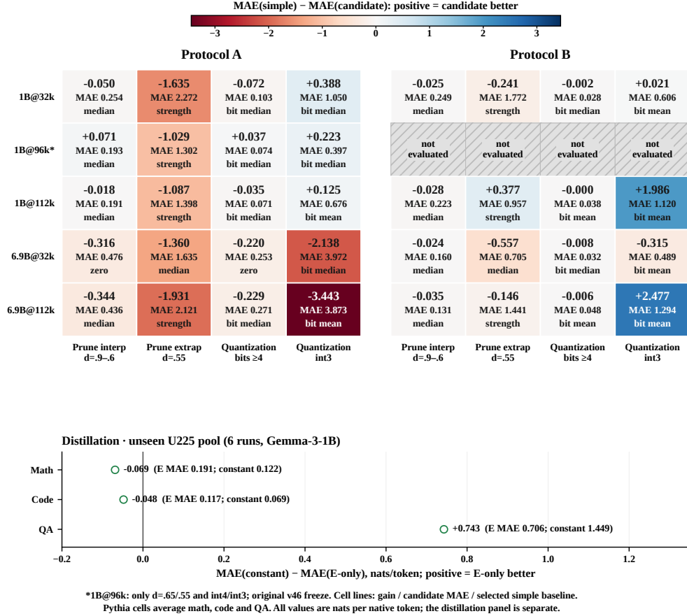
Figure 3: Generalization to unseen configurations and states. Top: improvement of the headline candidate over the strongest source-free reference (MAE difference, nats, averaged over the three capabilities; positive = candidate better) for each new source (rows), regime (columns), and fitting protocol (panels), with the candidate MAE printed in each cell; the confirmation panel (410M@48k, 1.4B@112k, 6.9B@80k) and the grouped-quantization tests are included. Cells not evaluated are hatched. Bottom: the distillation pool test, reuse-count form against the constant on the unseen pool U225, per capability. All predictions were frozen before the corresponding measurement.
