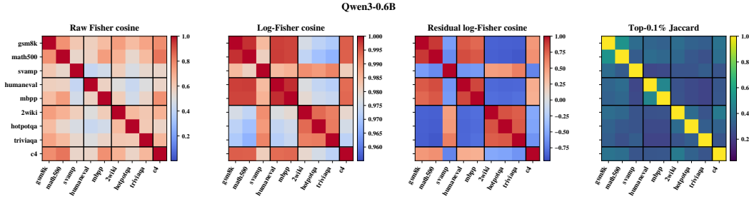
Figure 6: Capability regions in gradient space for Qwen3-0.6B: pairwise similarity of per-benchmark gradient signatures under four metrics (raw Fisher cosine, log-Fisher cosine, shared-component-removed log-Fisher cosine, top-0.1% coordinate Jaccard). Black lines separate the math, code, QA, and control blocks.
