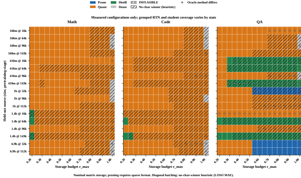
Figure 16: Capability-specific selection maps on held-out Pythia states. For each held-out state (rows, ordered by size and stage) and nominal storage budget r_{\max} (columns), the colour is the method whose law-predicted loss is lowest among the measured configurations within budget (pruning r = d , per-channel RTN r = b/16 , grouped RTN r = (b + 16/g)/16 , distillation to a smaller same-stage student r = N_S/N_0 ; the dense source at r = 1 ); every law is refit with the state held out. Grey cross-hatching marks cells with no feasible configuration for a policy; diagonal hatching marks cells in which the predicted gap between the two best methods is smaller than the larger of their leave-one-state-out errors (a heuristic); a marker shows where the measured oracle chooses a different method. Nominal pruning storage requires a sparse format. Generated by v64_selection_feasible.py.
