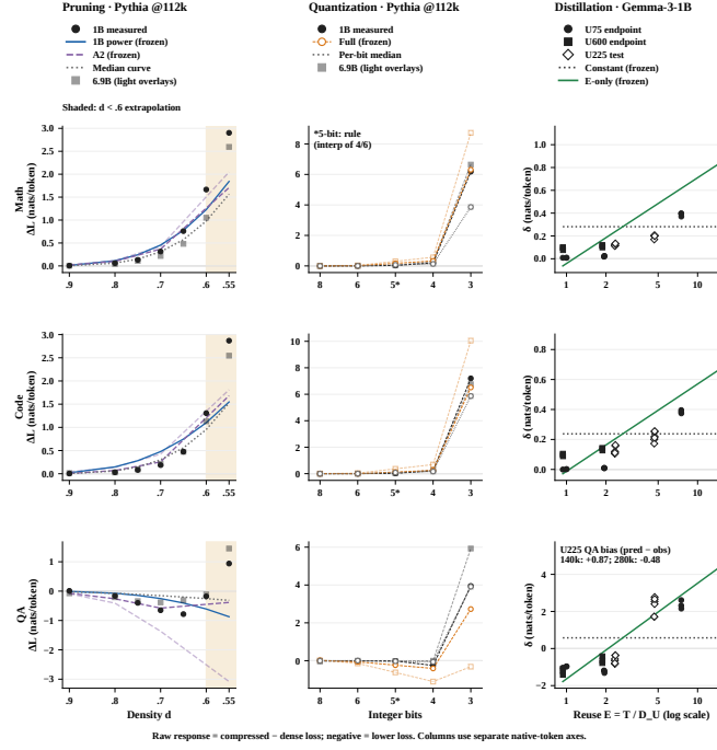
Figure 1: Capability-conditioned compression responses and frozen predictions, one source per arm. Left: pruning of Pythia-1B at step 112k (measured, filled circles) with the frozen power form (Eq. 3), the per-density regression A2, and the source-free median curve; the 6.9B source is overlaid in grey and the extrapolated density 0.55 is shaded. Middle: per-channel quantization of the same sources with the frozen per-bit regression (hollow) and the per-bit median (dotted). Right: distillation of Gemma-3-1B, signed transfer \delta_c against the reuse count E ; endpoint pools (fit) and the unseen pool U225 (test) with the frozen constant and reuse-count forms. Lines are fits frozen before the test points were measured; native nats per token.
