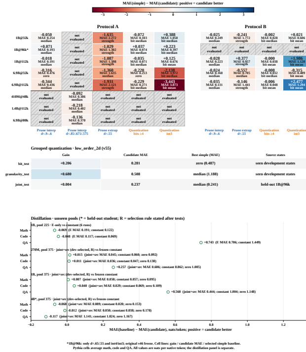
Figure 2: Generalization to unseen configurations and states. Top: improvement of the headline candidate over the strongest source-free reference (MAE difference in nats, averaged over capabilities; positive = candidate better) per new source (rows), regime (columns), and fitting protocol (panels), with the candidate MAE in each cell; hatched cells were not evaluated. Bottom: the distillation pool tests per capability against the frozen constant. All predictions were frozen before the corresponding measurement.
