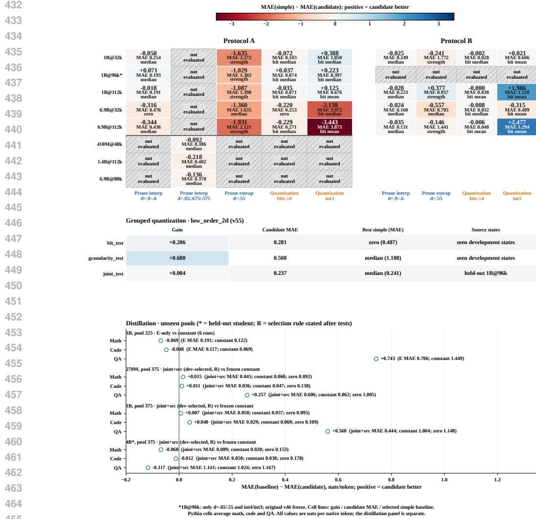
Figure 2: Generalization to unseen configurations and states. Top: improvement of the headline candidate over the strongest source-free reference (MAE difference, nats, averaged over the three capabilities; positive = candidate better) for each new source (rows), regime (columns), and fitting protocol (panels), with the candidate MAE printed in each cell; the confirmation panel (410M@48k, 1.4B@112k, 6.9B@80k) and the grouped-quantization tests are included. Cells not evaluated are hatched. Bottom: the distillation pool test, reuse-count form against the constant on the unseen pool U225, per capability. All predictions were frozen before the corresponding measurement.
