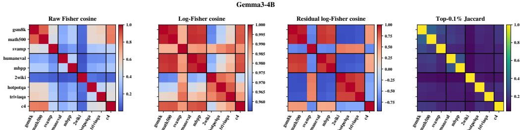
Figure 12: Capability regions in gradient space for Gemma3-4B: pairwise similarity of per-benchmark gradient signatures under four metrics (raw Fisher cosine, log-Fisher cosine, shared-component-removed log-Fisher cosine, top-0.1% coordinate Jaccard). Black lines separate the math, code, QA, and control blocks.
