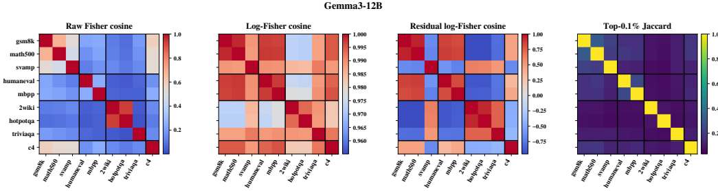
Figure 4: Capability regions in gradient space for Gemma3-12B: pairwise similarity of per-benchmark gradient signatures under four metrics (raw Fisher cosine, log-Fisher cosine, shared-component-removed log-Fisher cosine, top-0.1% coordinate Jaccard). Black lines separate the math, code, QA, and control blocks.
