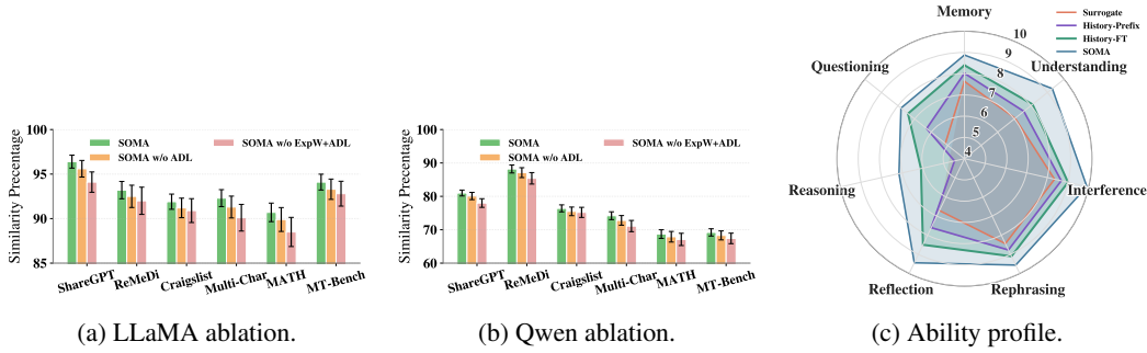
Figure 5: Component and capability analysis. Anti-degeneration regularization and expectation-weighted divergence both improve mining on LLaMA (a) and Qwen (b). (c) MT-Bench-101 ability profile of Surrogate , History-Prefix , History-FT , and SOMA .
