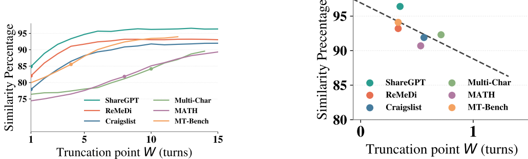
(a) Similarity under different switch points.
