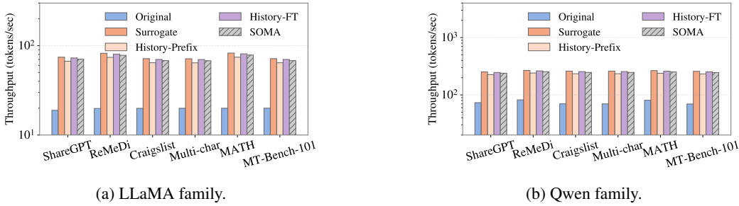
Figure 2: Throughput across six datasets. SOMA keeps the serving path close to the surrogate while maintaining higher similarity to the original model.
