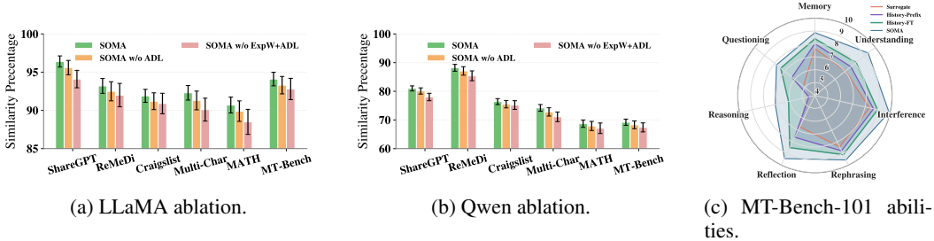
Figure 3: Component and capability analysis. Both anti-degeneration regularization and expectation-weighted divergence improve mining on LLaMA (a) and Qwen (b), and SOMA gains across MT-Bench-101 abilities (c).
