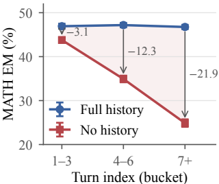
(a) Later turns depend on context
