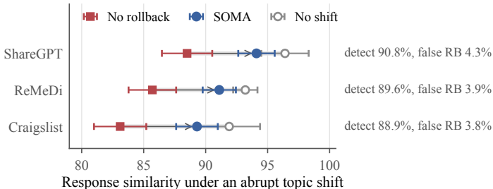
(b) Rollback recovers most of the drop
