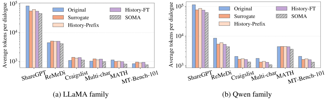
Figure 10: Average tokens per dialogue across six datasets. SOMA reduces token usage by avoiding repeated full-history serving after switching.
