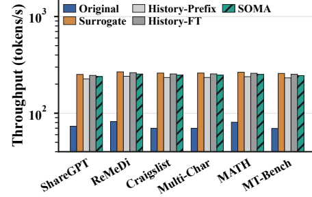
(b) Qwen family.
