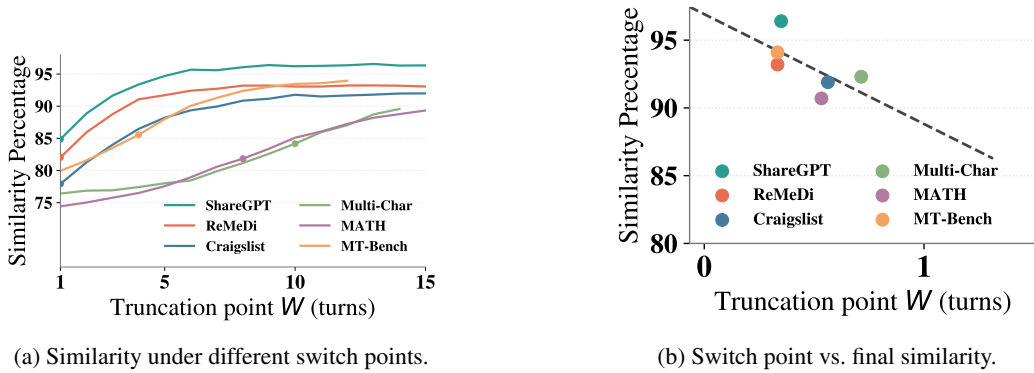
Figure 4: Warm-start and switching behavior. Easier local-dialogue settings switch earlier, while reasoning-heavy or multi-party settings need longer warm starts and achieve lower final similarity.
