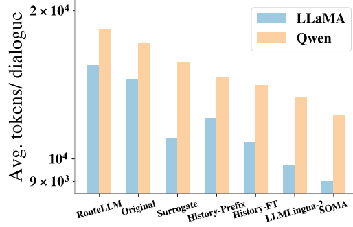
Figure 7: Average tokens per dialogue for SOMA on both model families across the six datasets.
