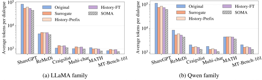
Figure 8: Average tokens per dialogue across six datasets. SOMA reduces token usage by avoiding repeated full-history serving after switching.
