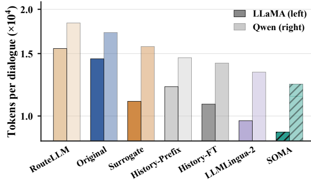
Figure 9: Average tokens per dialogue of each method on both model families.
