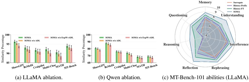
Figure 5: Component and capability analysis. Anti-degeneration regularization and expectation-weighted divergence both improve mining on LLaMA (a) and Qwen (b). (c) MT-Bench-101 ability profile of Surrogate , History-Prefix , History-FT , and SOMA .
