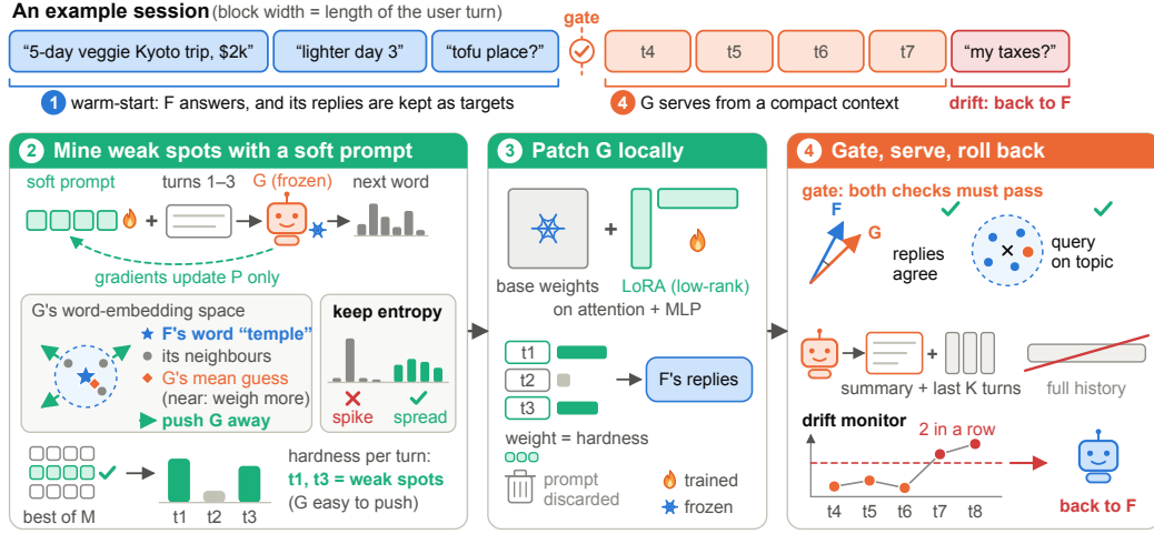
Figure 2: Overview of SOMA on an example session (top; block width is the length of the user turn, color shows who serves it). (1) F answers the warm-start turns, and its replies become targets. (2) A soft prompt on the frozen surrogate G pushes G 's next-word mass away from F 's words and their embedding neighbors under an entropy guard; the best of M prompts scores how hard each turn is. (3) A LoRA adapter is fitted to F 's replies with these hardness weights, and the prompt is discarded. (4) A gate switches to G when its replies agree with F and the query stays on topic; G then serves from a summary plus the last K turns until a drift monitor rolls back to F .
