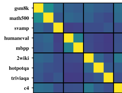
Top-0.1% Jaccard
