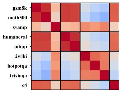
Log-Fisher cosine
