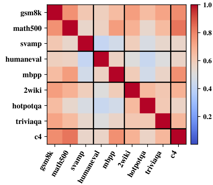
Raw Fisher cosine
