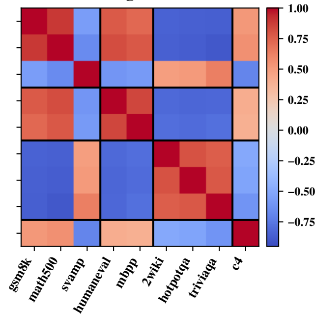
Residual log-Fisher cosine
