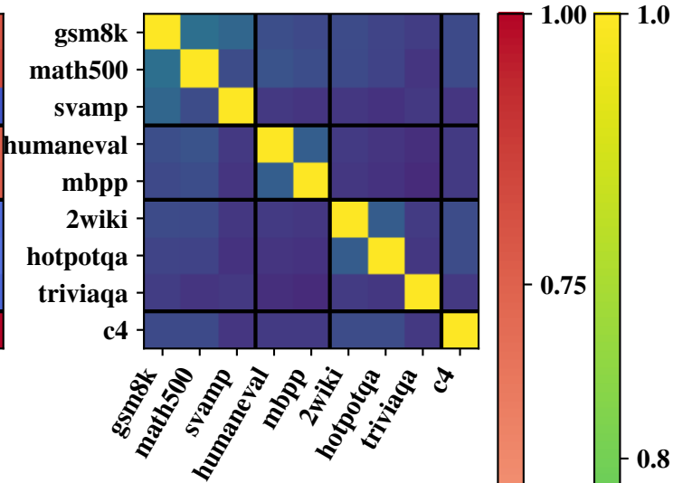
Top-0.1% Jaccard
