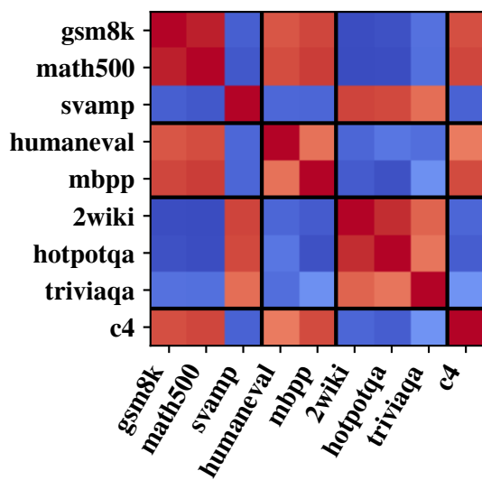
Muse-30B
