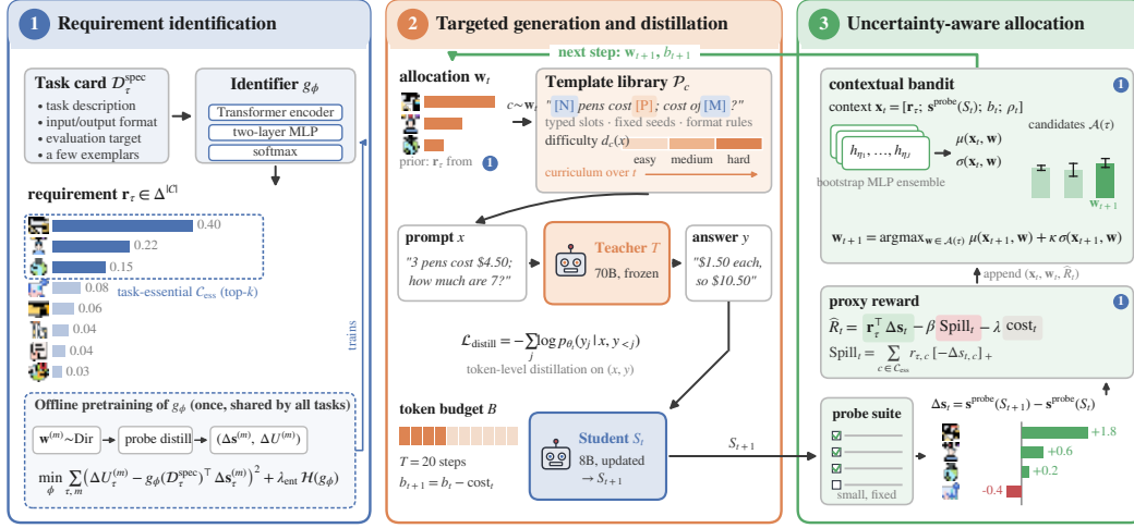
Figure 2: Overview of ReAD. (1) An identifier g_\phi , pretrained once on low-budget probe interventions, maps a task card to the requirement vector \mathbf{r}_\tau , whose top- k entries form C_{\text{ess}} . (2) At step t , capabilities are sampled from the allocation \mathbf{w}_t , prompts are instantiated from typed templates under a difficulty curriculum, and the student is distilled on the teacher’s answers. (3) The probe-profile change \Delta \mathbf{s}_t gives the proxy reward, which trains a bootstrap ensemble whose mean \mu and uncertainty \sigma select \mathbf{w}_{t+1} by UCB; the loop repeats until B is spent. Values in the figure are illustrative.
