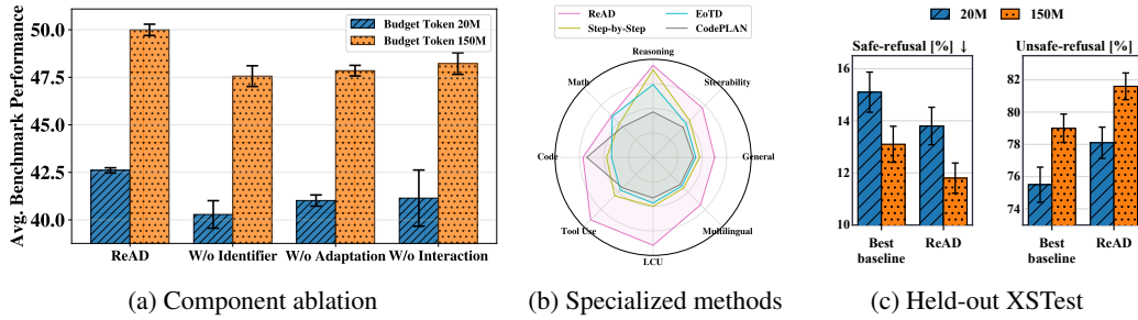
Figure 5: (a) Component ablation (average score over eight capabilities). (b) ReAD vs. step-by-step distillation, EoTD, and CodePLAN at 150M (fraction of the teacher–student gap closed). (c) XSTest refusal rates of ReAD and the best SFT/KD baseline.
