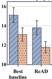
Safe-refusal [%] ↓
