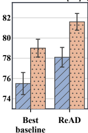
Unsafe-refusal [%] ↑
