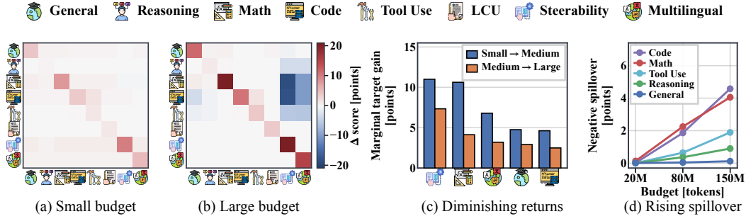
Figure 1: Exploratory study. (a–b) Cross-capability transfer under single-capability distillation. Larger budgets sharpen target gains and tend to expose stronger negative transfer. (c–d) Budget waste. Extra tokens yield smaller target gains and more spillover to non-target capabilities.
