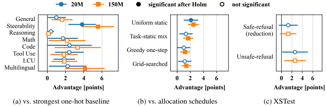
Figure 3: ReAD’s advantage with unadjusted 95% Welch intervals from the reported means and standard deviations (three seeds; blue circles 20M, orange squares 150M). Filled markers stay significant after Holm correction per panel and budget. Safe-refusal is shown as a reduction, so positive values favor ReAD in all panels.
