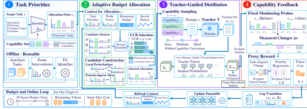
Figure 2: Overview of ReAD. (1) A pretrained identifier sets the task’s capability priorities \mathbf{r}_\tau . ReAD then repeats three steps until the budget B is spent: (2) a bandit selects the allocation \mathbf{w}_t by UCB; (3) the student is distilled on teacher outputs for prompts sampled from \mathbf{w}_t ; (4) the measured capability change yields a proxy reward that updates the bandit.
