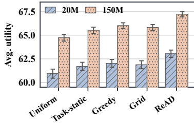
(c) Allocation schedules
