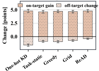
(a) Gain vs. spillover, 150M
