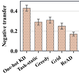
(b) Harmful transfer, 150M
