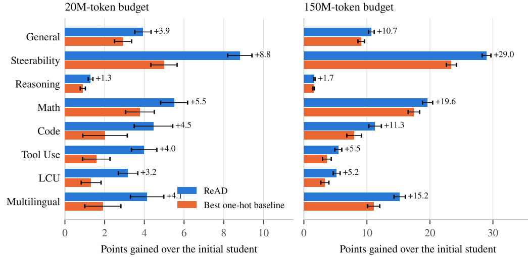
Figure 4: Points gained over the initial student on each capability at 20M (left) and 150M (right) for ReAD and for the best one-hot baseline of that capability, read off Table 1. Error bars are the standard deviation over three seeds of the distilled student’s score. Values are absolute percentage points, so small changes stay small.
