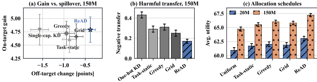
Figure 4: Budget-allocation diagnostics (mean \pm std, three seeds; values in Appendix Table 8). (a) On-target gain vs. off-target change and (b) negative transfer at 150M; (c) allocation schedules.
