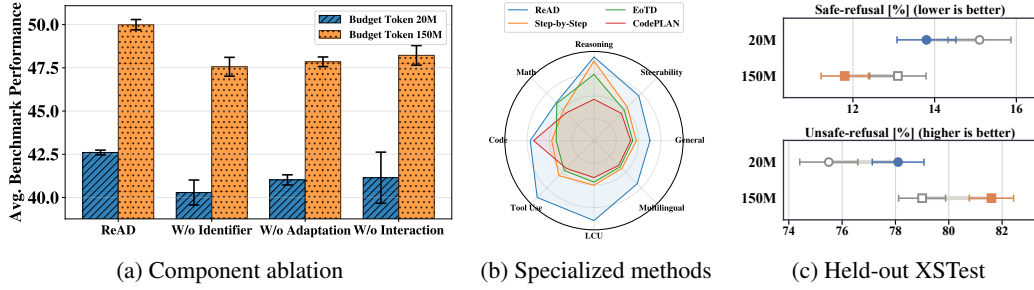
Figure 4: (a) Ablation of ReAD components: average benchmark score over the eight capabilities at 20M and 150M tokens. (b) ReAD versus step-by-step distillation, EoTD, and CodePLAN at 150M; axes show the fraction of the teacher–student gap closed per capability. (c) XSTest scores of ReAD (filled) and the best SFT/KD baseline (hollow), mean \pm std over three seeds; blue circles are 20M and orange squares 150M, as in (a).
