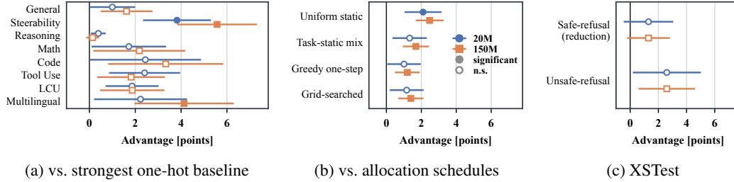
Figure 5: ReAD’s advantage with unadjusted 95% Welch intervals from the reported means and standard deviations (three seeds; blue circles 20M, orange squares 150M). Filled markers stay significant after Holm correction per panel and budget; safe-refusal is shown as a reduction, so positive values favor ReAD in all panels.
