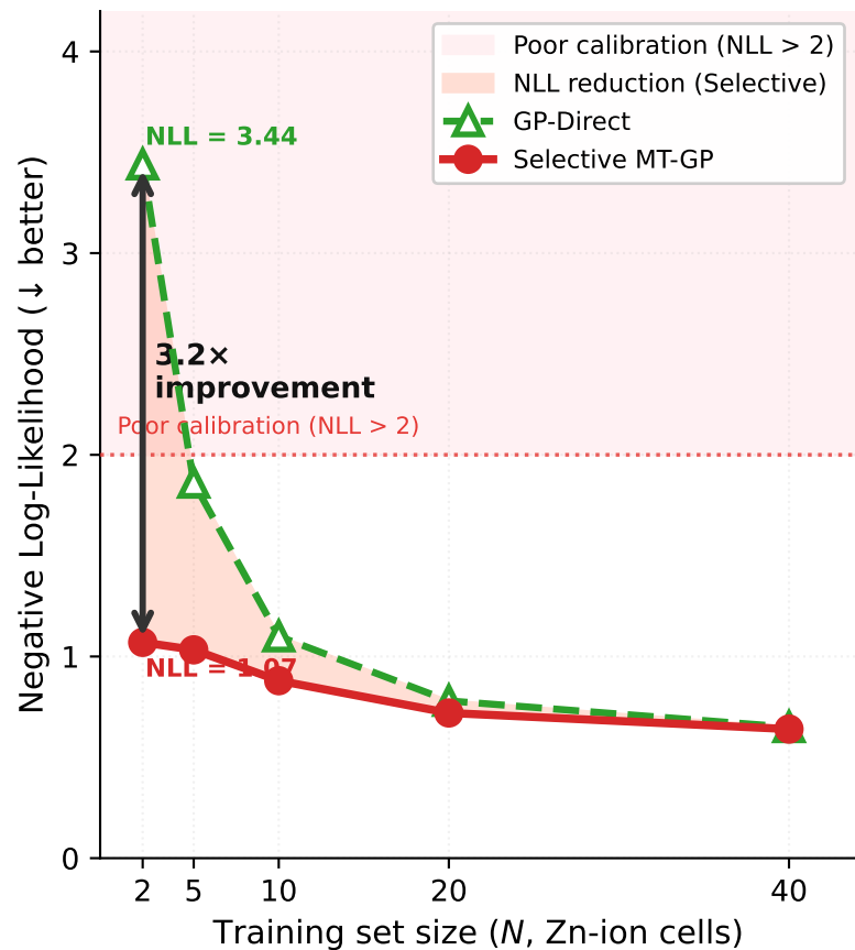
(b) Predictive Sharpness (NLL)
