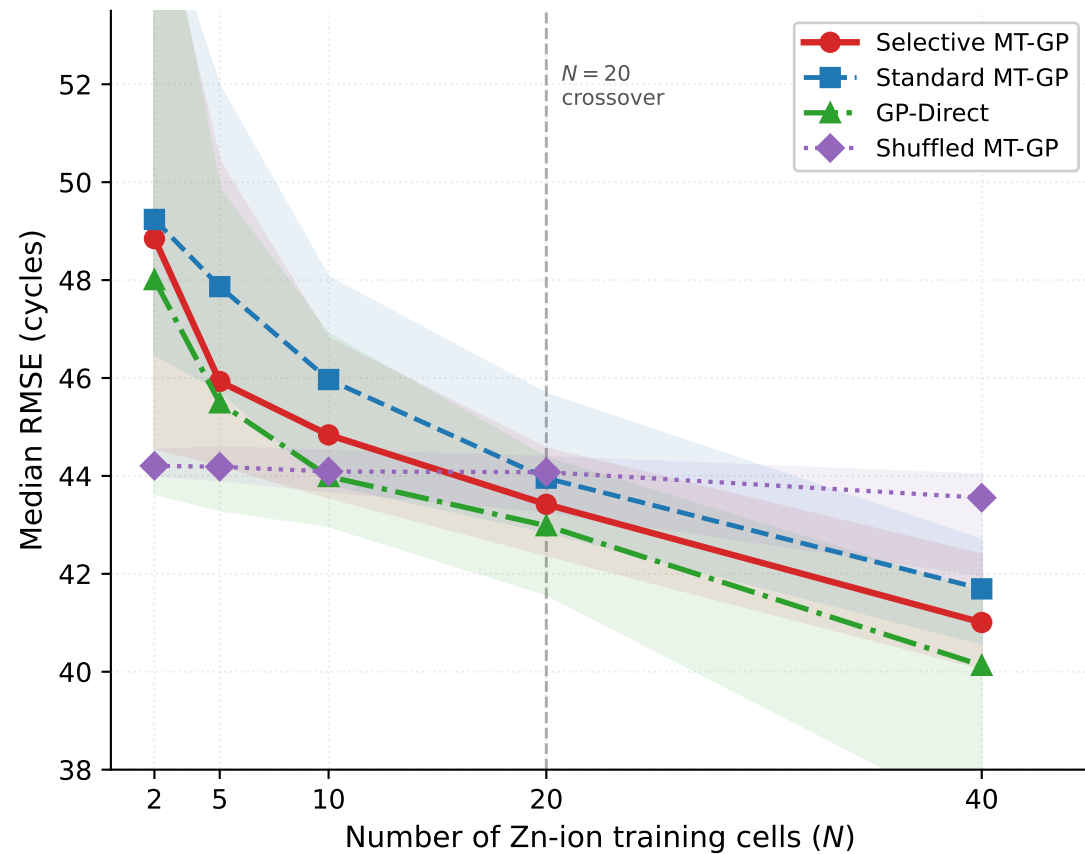
RMSE Comparison — 200 MC Trials (IQR bands)
