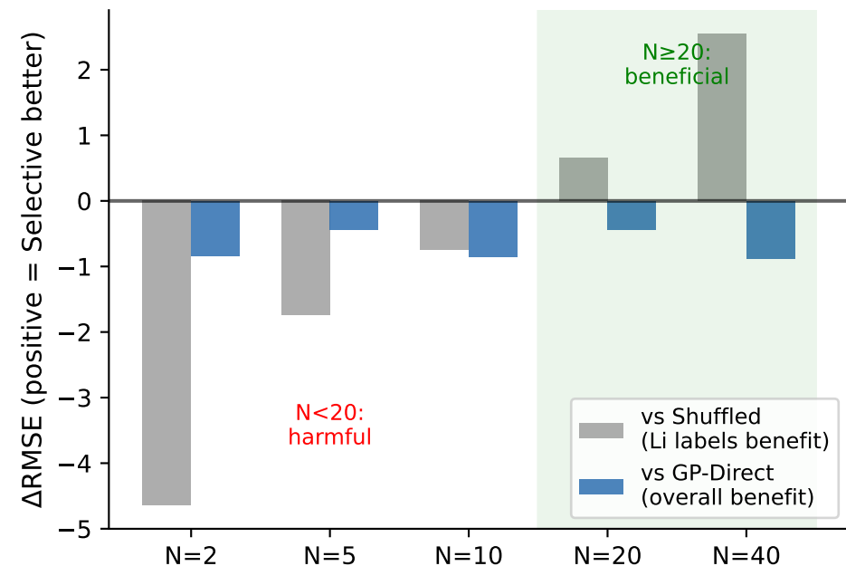
(C) When Does Transfer Help? [+value = Selective MT-GP wins]
