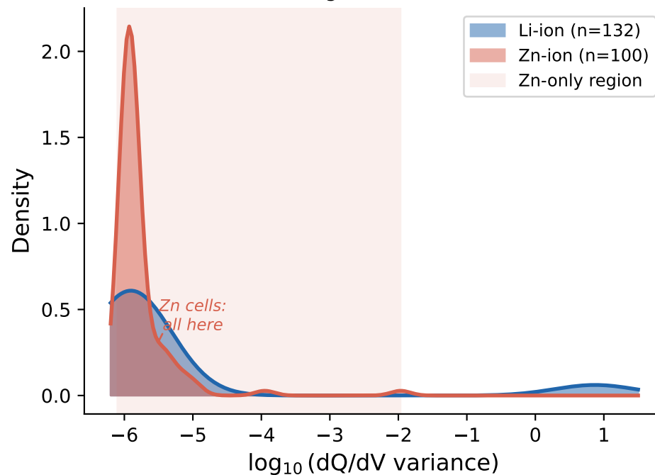
(B) Feature Distribution After Log Transform
