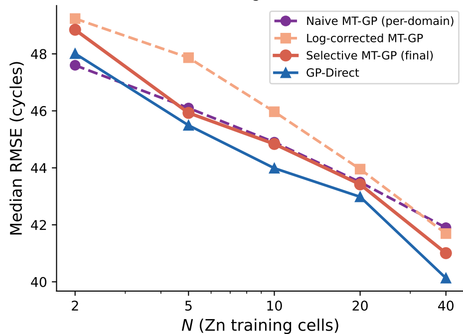
(A) Engineering Improvement: Naive → Log → Selective
