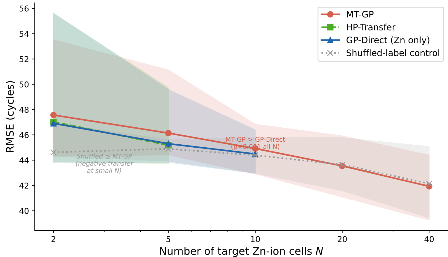
Cycle Life Prediction: Cross-Chemistry Transfer Learning
