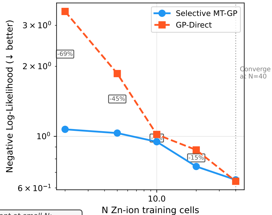
(C) Calibration: NLL
