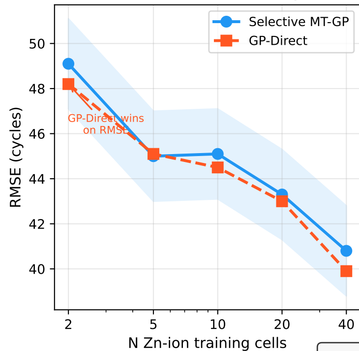
(A) Predictive Accuracy
