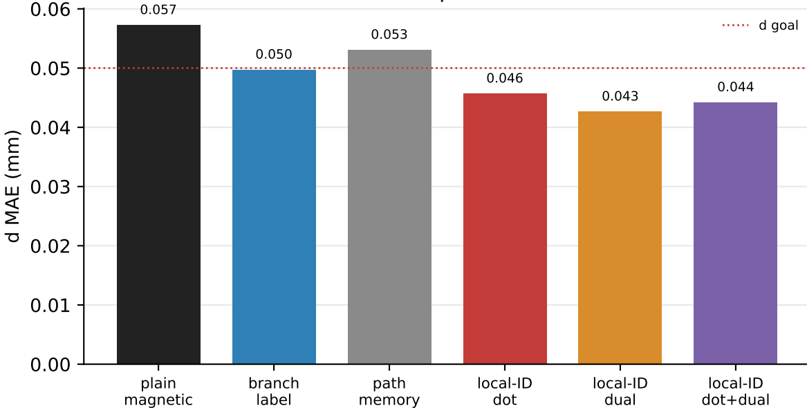
b Held-out displacement error
