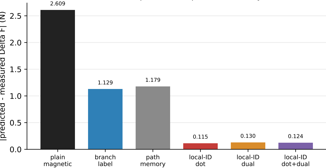
c Same-d pair force-split consistency
