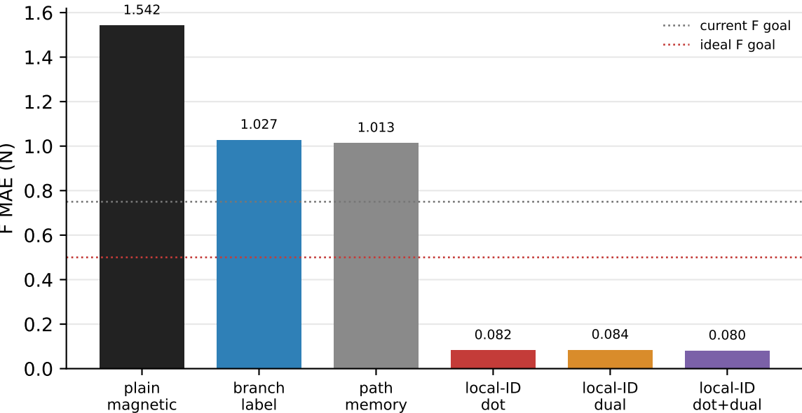
a Held-out force error
