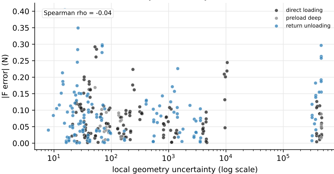
d Geometry uncertainty vs force error
