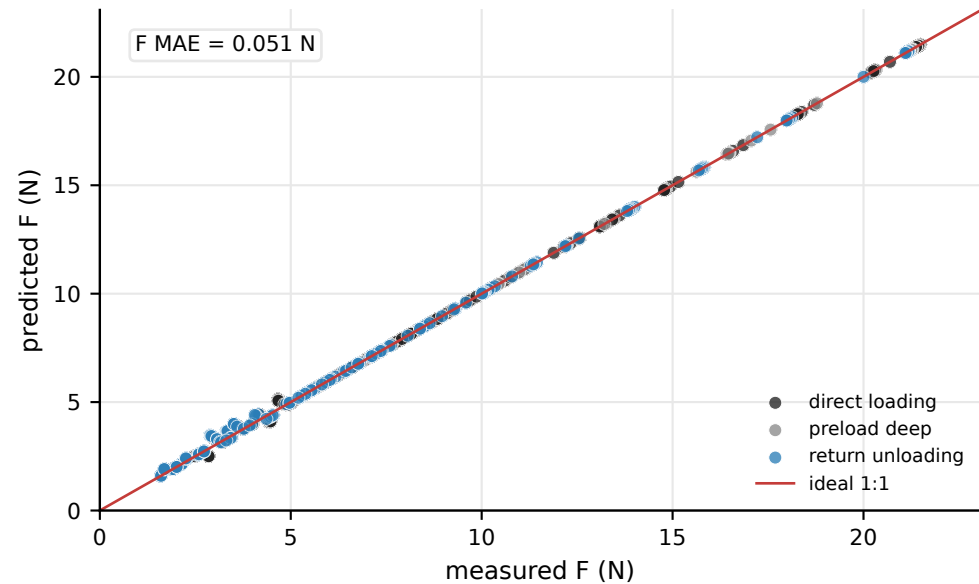
a Best linear estimator for force: Huber
