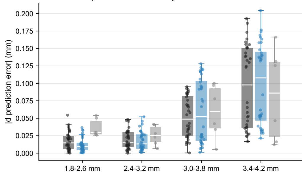
Displacement residual by work zone and branch
