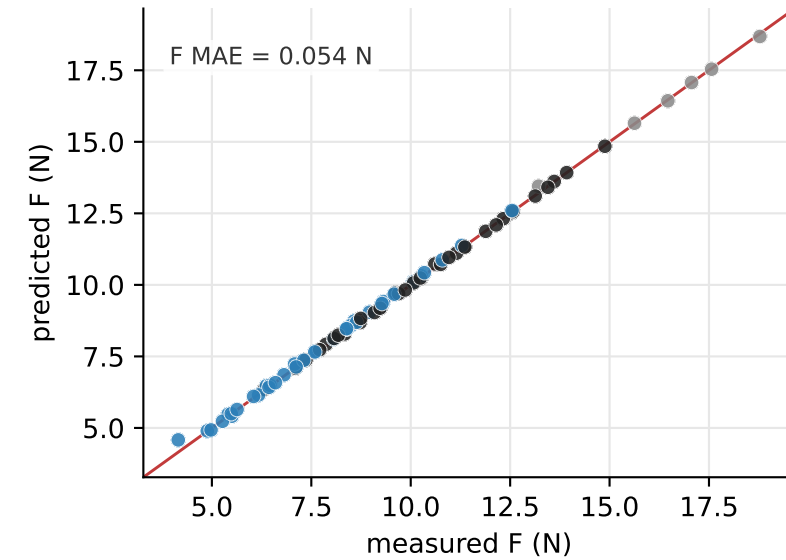
f Local-ID model B + path history + local jF/jd
