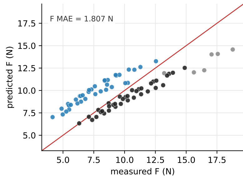
e Plain magnetic baseline B only
