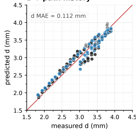
g Path-memory MLP B + path history
