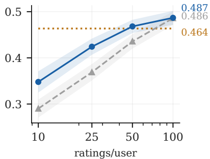
PLCC
