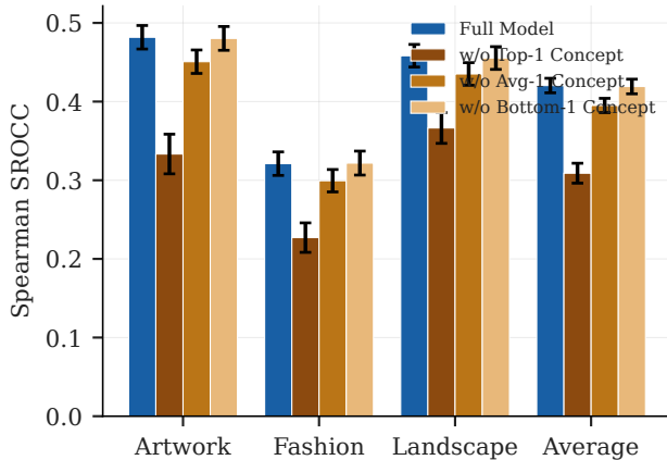
(b) Concept Ablation (Importance)
