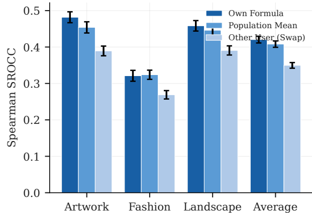
(a) Formula Swap (Personalization)
