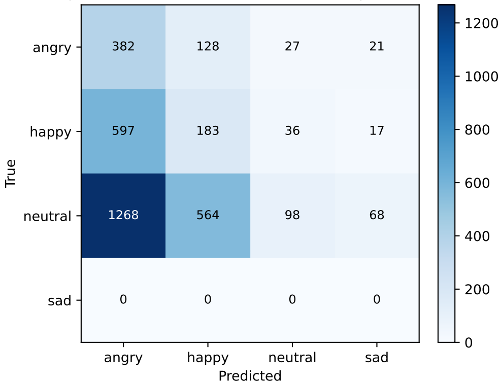
Exp4 Zero-Shot C-BESD→FAU (test-only, N=3389)
