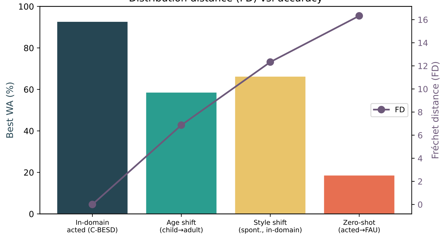
Distribution distance (FD) vs. accuracy
