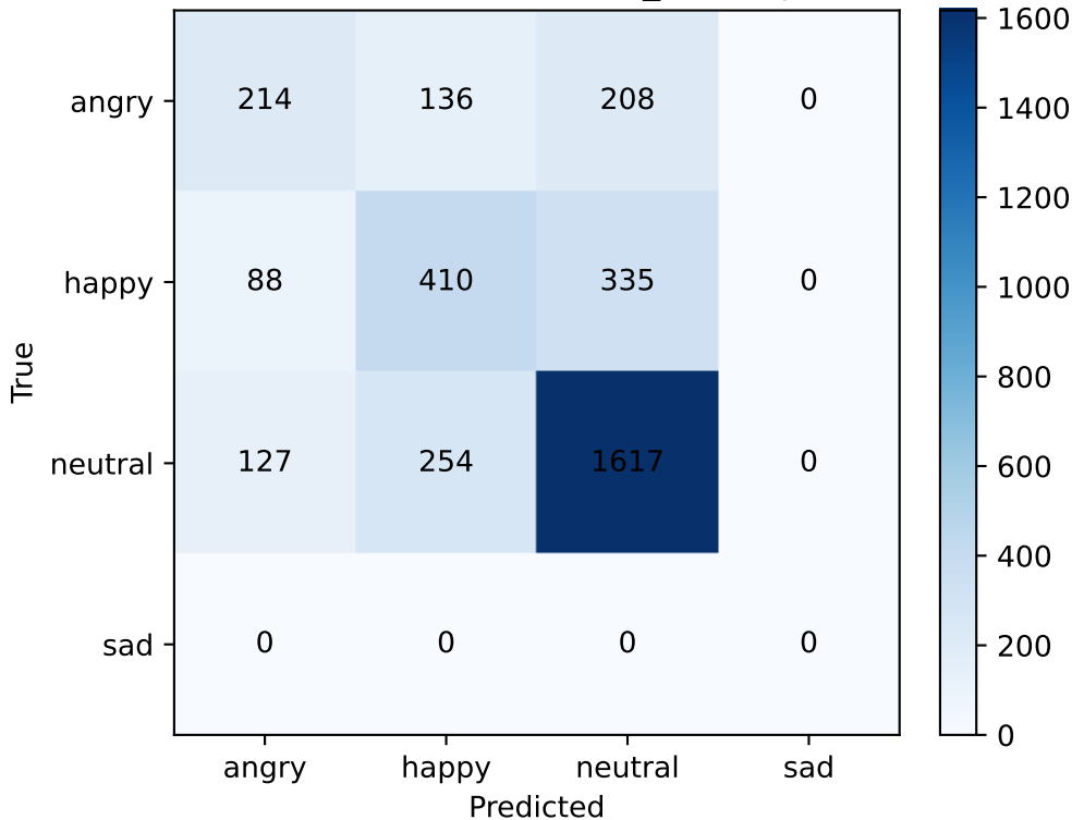
Confusion matrix (best_model.pt)
